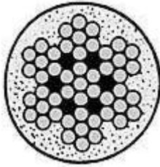
7 x 7 (Shown Vinyl Coated)
